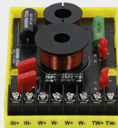
GZCX 165-200.2SQL 2-way high-power competition crossover also available separately
